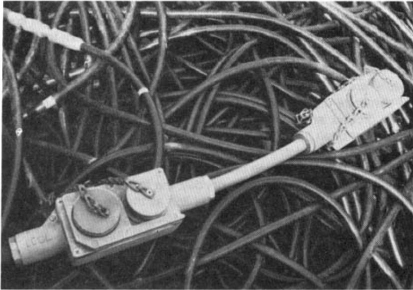
Seismic cable. Note cableheads.
